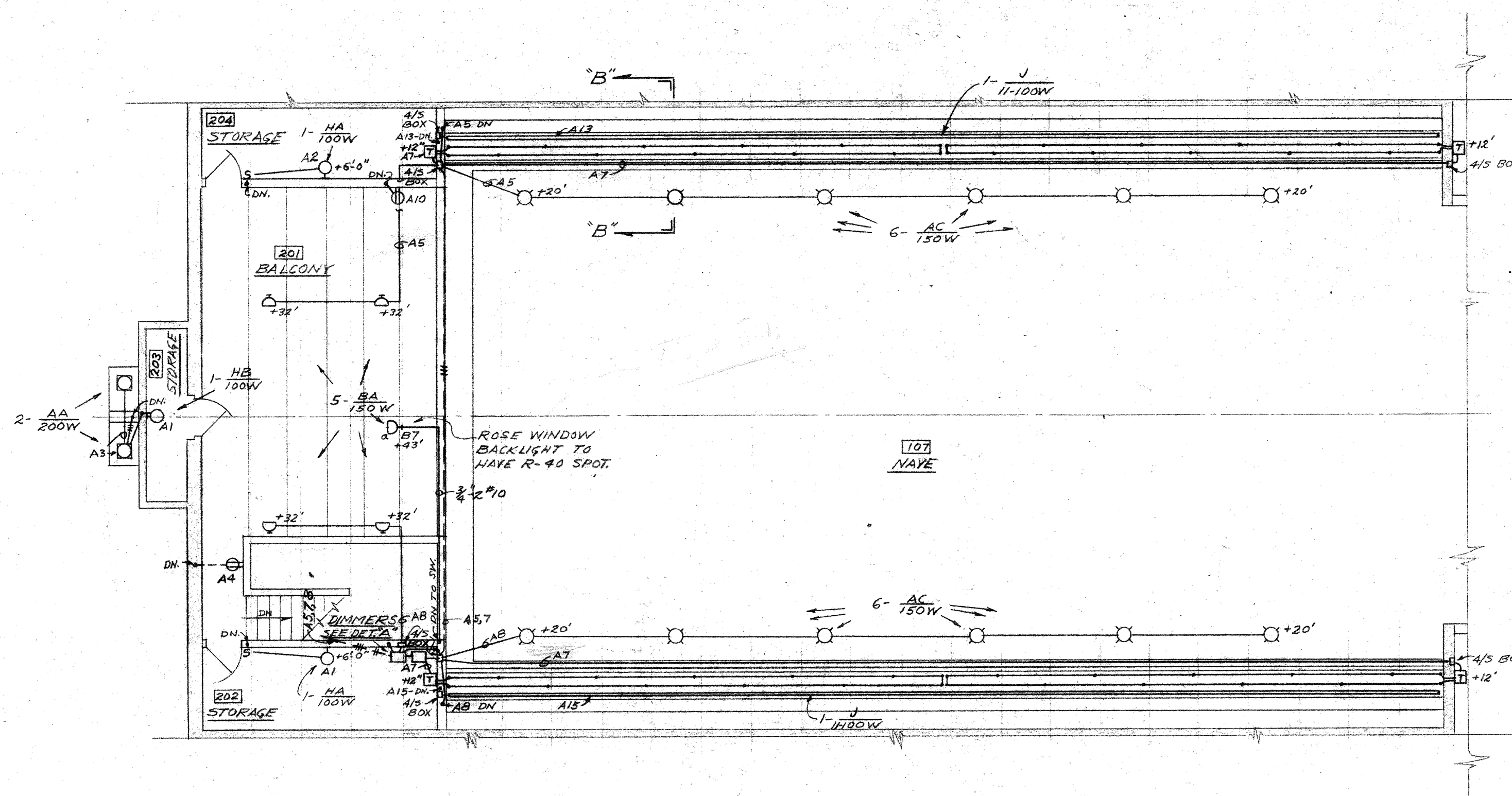
PLAN - BALCONY & LIGHT COVES SCALE: 1/8" = 1'-0"
